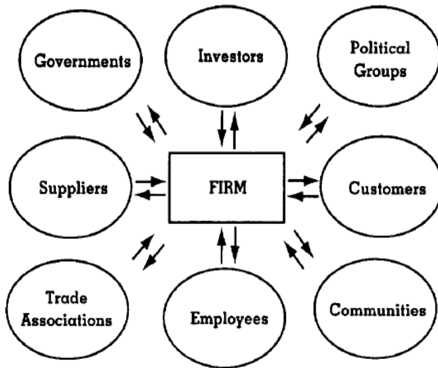
Figure 1: Stakeholder Theory
